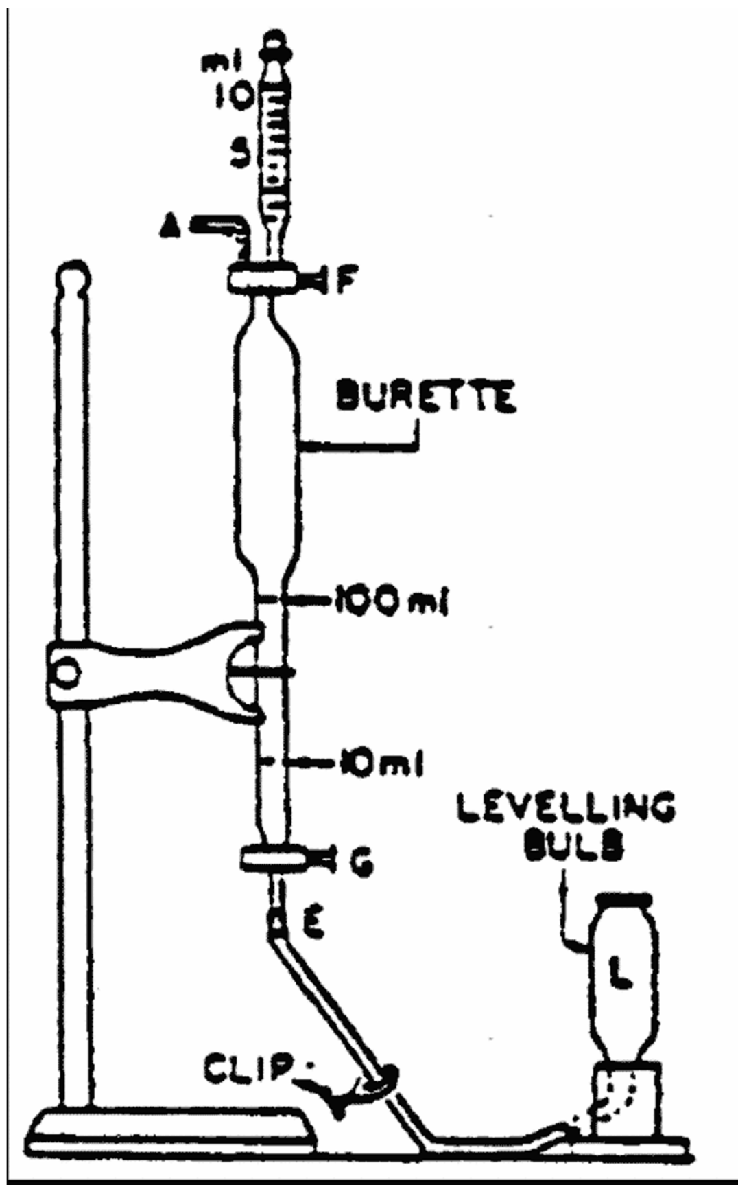
Figure 1. Tutwiler burette (lettered items mentioned in
